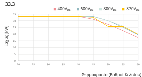
Fronius Verto 33.3
